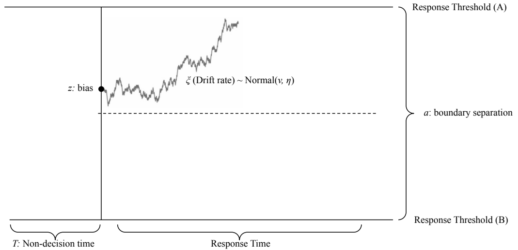
Figure 17. Simplified illustration of the drift-diffusion model. On every trial, after a period of time ( T ), an evidence accumulation process is initiated from the specified position ( z ) relative to the whole boundary separation ( a ). Evidence is gathered stochastically according to the drift rate ( \xi ) that follows a normal distribution with the mean \nu and the standard deviation \eta . When enough information is accumulated to cross one of the thresholds, a decision is made
