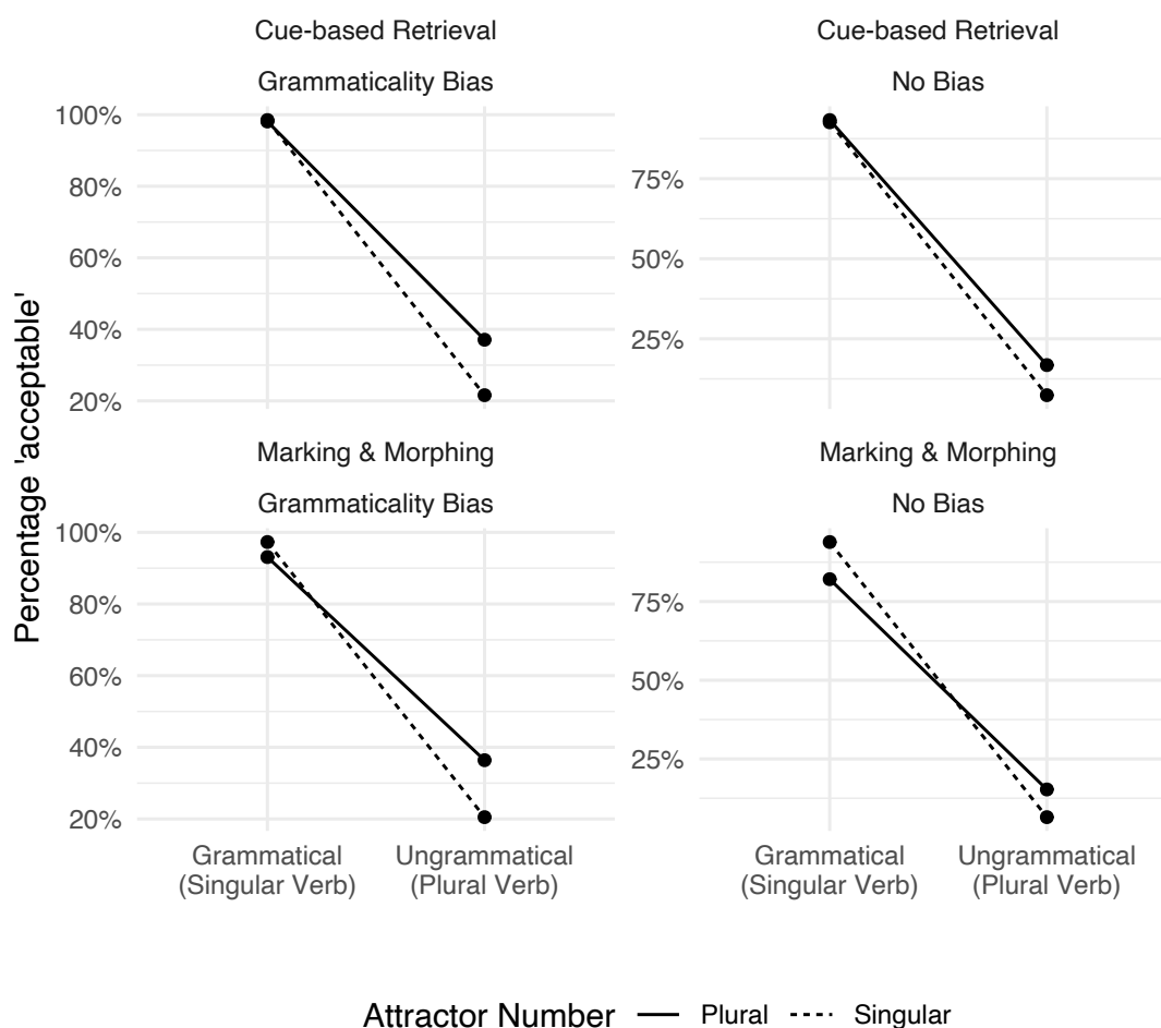
Figure 18. Drift Diffusion Model predictions in which the drift rate is manipulated according to the assumptions of agreement attraction accounts along with a bias manipulation
