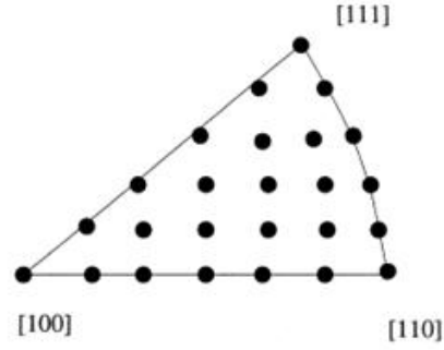
Figure 3.13. Stereographic projection of grain orientations forming up the martensite zone ahead of crack tip [56].
