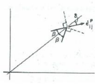
Figure 2.28. Angle between \dot{\epsilon}_{ij}^p and s_{ij} [53].
