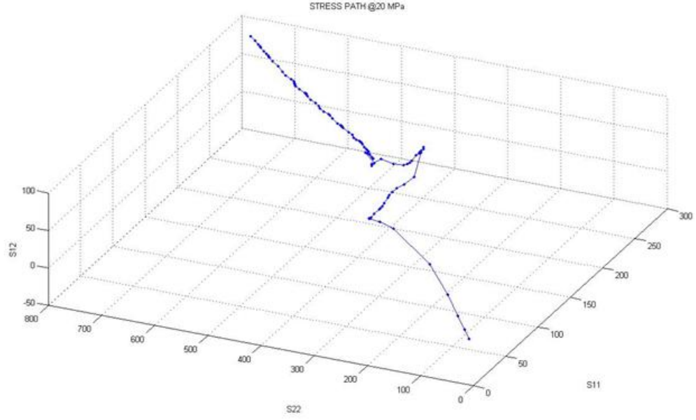
Figure 2.29. For \sigma^\infty = 20\text{MPa} and \frac{a}{B} = \frac{50}{100} , the stress path traversed in deviatoric stress space.
